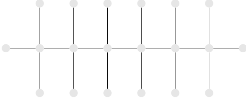
FIGURE 6. Graph DComb_8^{2+}
