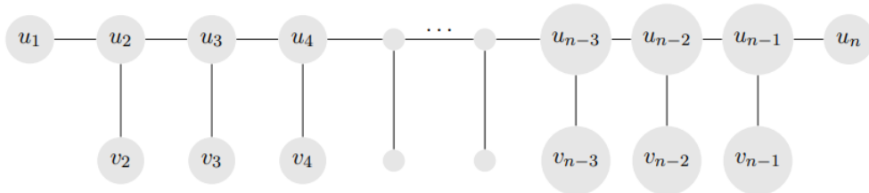
FIGURE 1. Graph Comb_n^{2+}
