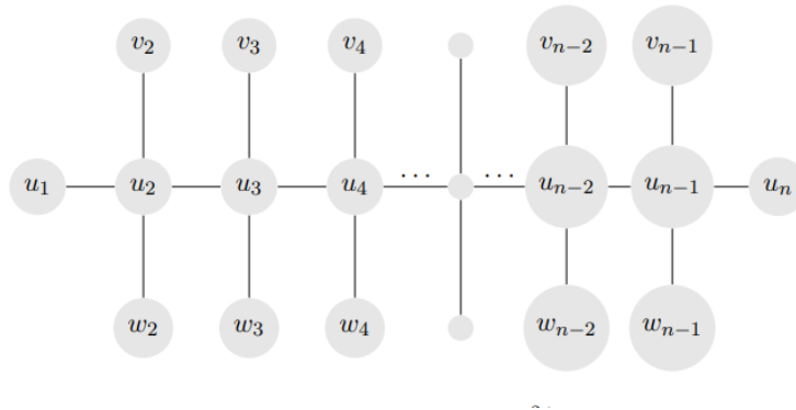
FIGURE 5. Graph DComb_n^{2+}
